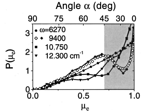
Fig. 4. Photon escape function as a function of the cosine \mu_e of the escape angle \alpha for an inverse opal with lattice parameter a = 930 \text{ nm} for frequencies \omega = 6270, 9400, 10,750, 12,300 \text{ cm}^{-1} (filled circles, diamonds, squares, triangles, respectively) as extracted from a white-lamp data set. These frequencies correspond to a/\lambda = 0.58, 0.87, 1.0, \text{ and } 1.14 . Open diamonds show a measurement obtained from the same sample with a Nd:YVO laser beam ( \omega = 9400 \text{ cm}^{-1} ). An angular scale is shown on the top axis. The shaded region corresponds to half of the range of the exit angle \alpha relative to the surface normal. The dashed curve partially obscured by filled circles corresponds to calibration measurements on a dilute colloidal suspension.
