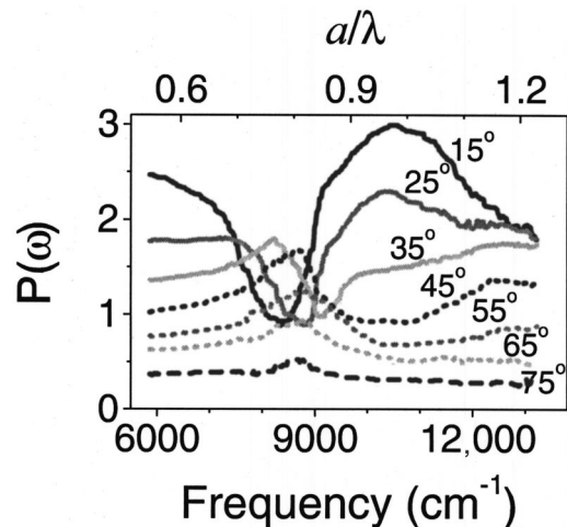
Fig. 3. Photon escape function as a function of frequency for an inverse opal with lattice parameter a = 930 \text{ nm} for exit angles \alpha = 15^\circ, 25^\circ, 35^\circ, 45^\circ, 55^\circ, 65^\circ, 75^\circ . The incidence angle is \gamma = 0^\circ . The top axis shows normalized frequency units a/\lambda where \lambda is the wavelength in vacuum. No relative scaling or offset was applied to the curves.
