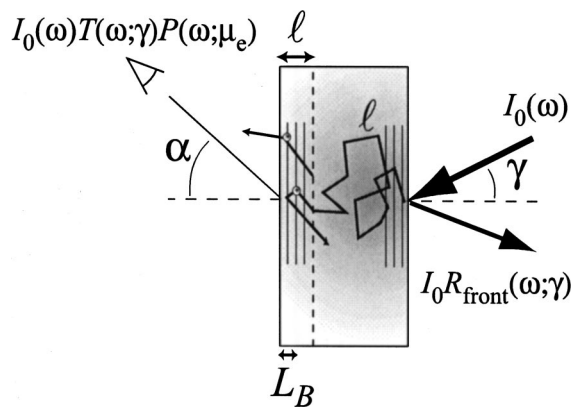
Fig. 1. As an incident light beam I_0(\omega) impinges on a photonic crystal, a fraction R_{\text{front}}(\omega; \gamma) is Bragg reflected, which depends on the frequency \omega and the angle of incidence \gamma . In the sample the light diffuses with typical step length \ell(\omega) . The diffuse glow on the transmission side is measured as a function of \cos \alpha = \mu_e . The depth of stop gaps in the escape function is determined by \ell and the Bragg attenuation length L_B (see Section 5).
