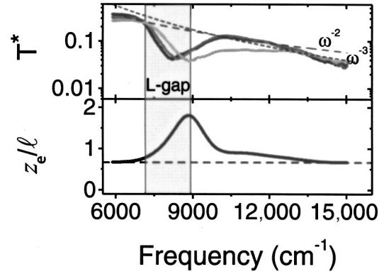
Fig. 8. \tau_e = z_e/\ell pertaining to the fit to the data in Fig. 5. Upper panel: T^* = T/(1 + \tau_e[1 - 2T]) for incidence angles \gamma = 0^\circ, 15^\circ, 30^\circ (black, dark gray, and light gray curves, respectively). Dashed curves represent the power laws \omega^{-3} (short dashes) and \omega^{-2} (long dashes).
